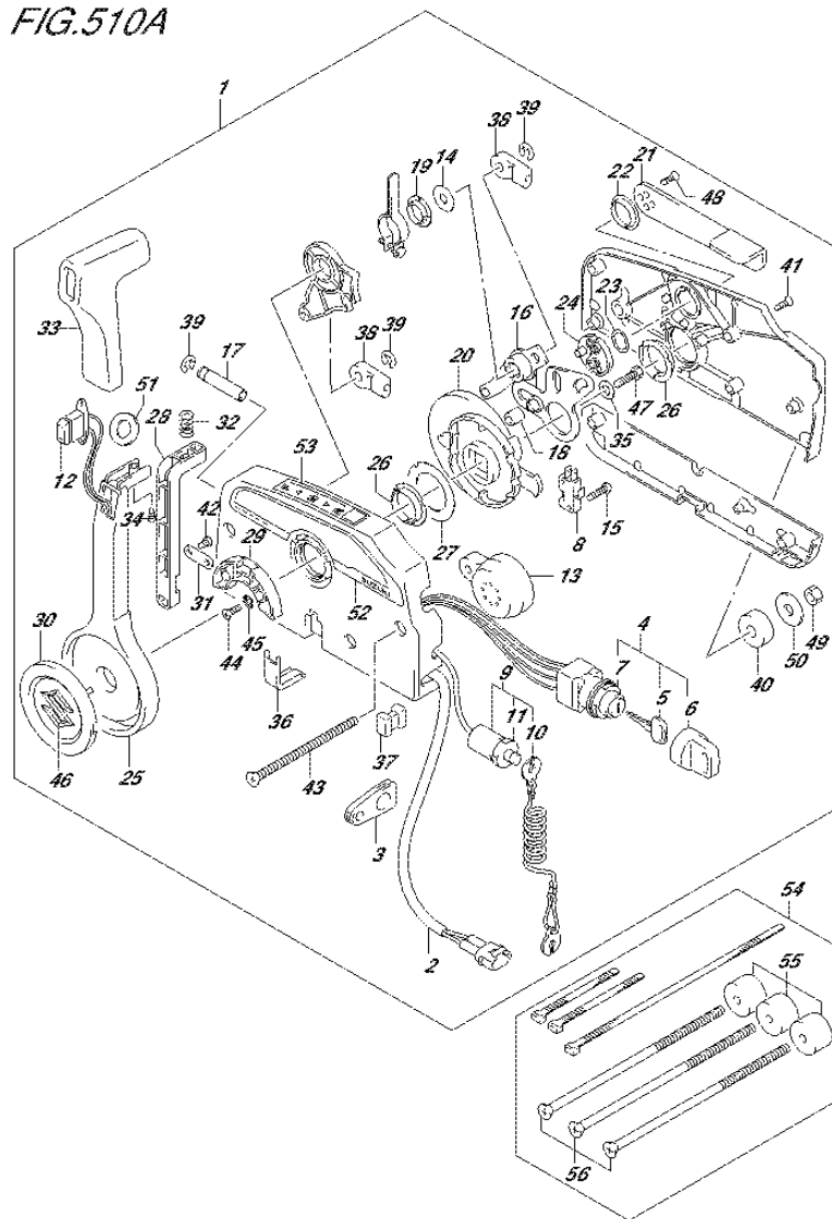
FIG.510A (3-E-5) OPT:REMOTE CONTROL (2) (DF100AT E11)
