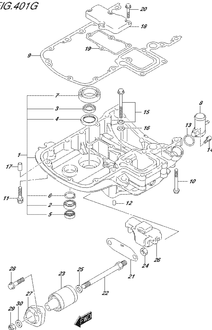
FIG.401G (2-G-5) ENGINE HOLDER (DF140AT E40)
