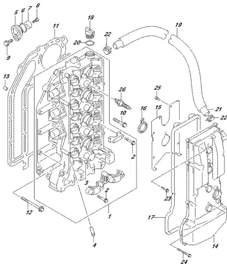
REF NO. PART NO. DESCRIPTION QTY REMARKS 1 11100-90J11 HEAD, CYLINDER 1 2 09103-06266 .BOLT (6X40) 21 3 09206-08001 .PIN (8X11) 18 4 11115-85FA1-001 GUIDE, VALVE (OS:0.3) 16 OPT 5 11261-93J00 COVER, PROTECTION ANODE 2 6 09280-22019 O RING (D:1.9,ID:21.8) 2 7 55321-87J01 ANODE, PROTECTION 2 8 09103-06281 BOLT (6X14) 2 9 01550-08207 BOLT 2 10 11117-89J00 BOLT, CYLINDER HEAD 10 11 11141-92J01 GASKET, CYLINDER HEAD 1 12 09116-08125 BOLT (8X50) 8 13 04211-13189 PIN 2 14 11170-90J11 COVER, CYLINDER HEAD 1 15 11173-90J00 PLATE, BREATHER 1 16 11179-90J00 GASKET, SPARK PLUG HOLE 4 17 11189-90J00 GASKET, CYLINDER HEAD COVER 1 18 11382-93J00 CAP, OIL FILLER 1 19 18498-90J20 PROTECTOR, BREATHER HOSE 1 20 09280-26006 O RING (D:3.1,ID:26.4) 1 21 09355-13207-00B HOSE (13X20X2000) 1 L:2000->660 22 09401-20409 CLIP 2 23 01547-06257 BOLT 11 24 01547-06557 BOLT 4 25 02112-0612A SCREW 7 26 09482-00427 SPARK PLUG (BKR6E) 4 NGK
