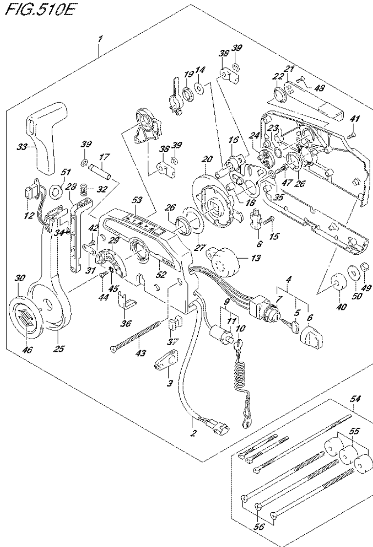
FIG.510E (3-F-5) OPT:REMOTE CONTROL (2) (DF115AZ E40)
