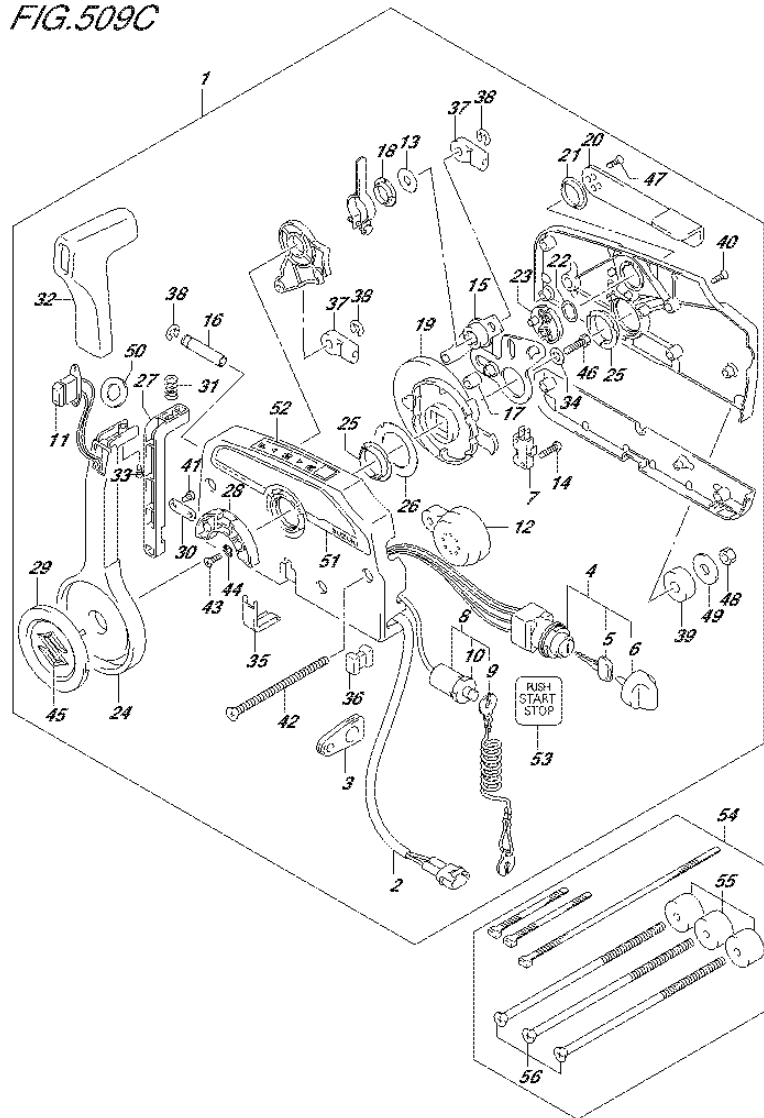
FIG.509C (3-D-12) OPT:REMOTE CONTROL (1) (DF115AZ E11)
