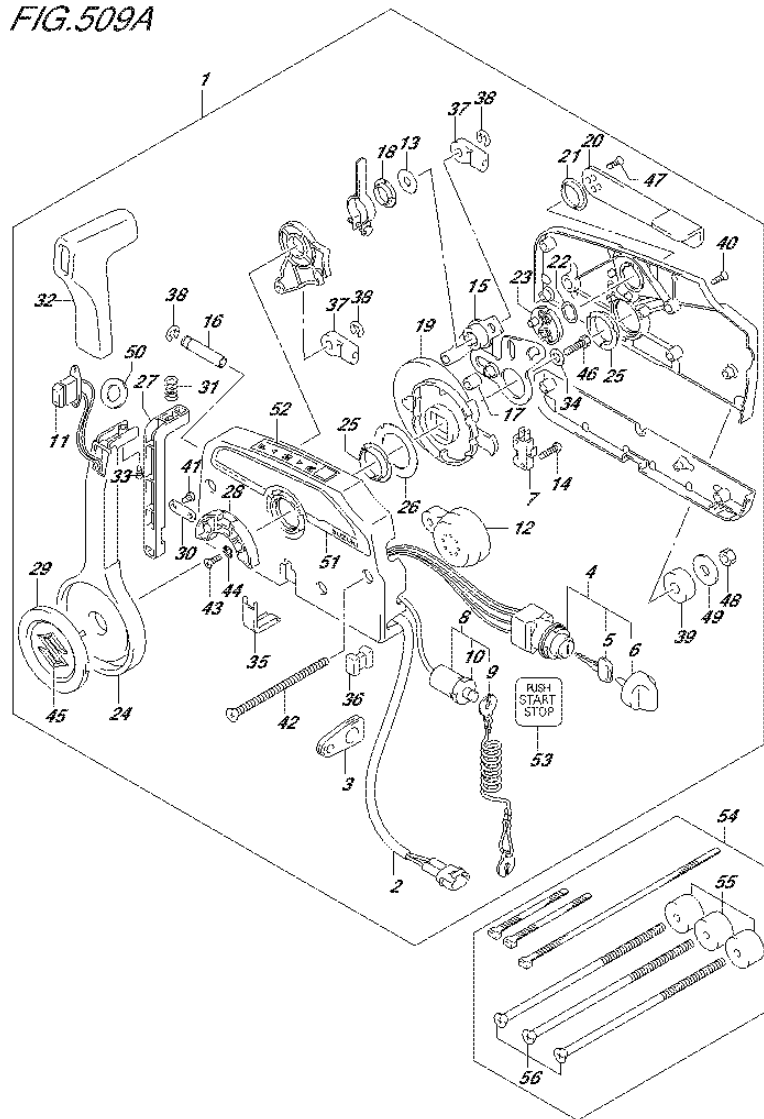
FIG.509A (3-D-5) OPT:REMOTE CONTROL (1) (DF100AT E11)
