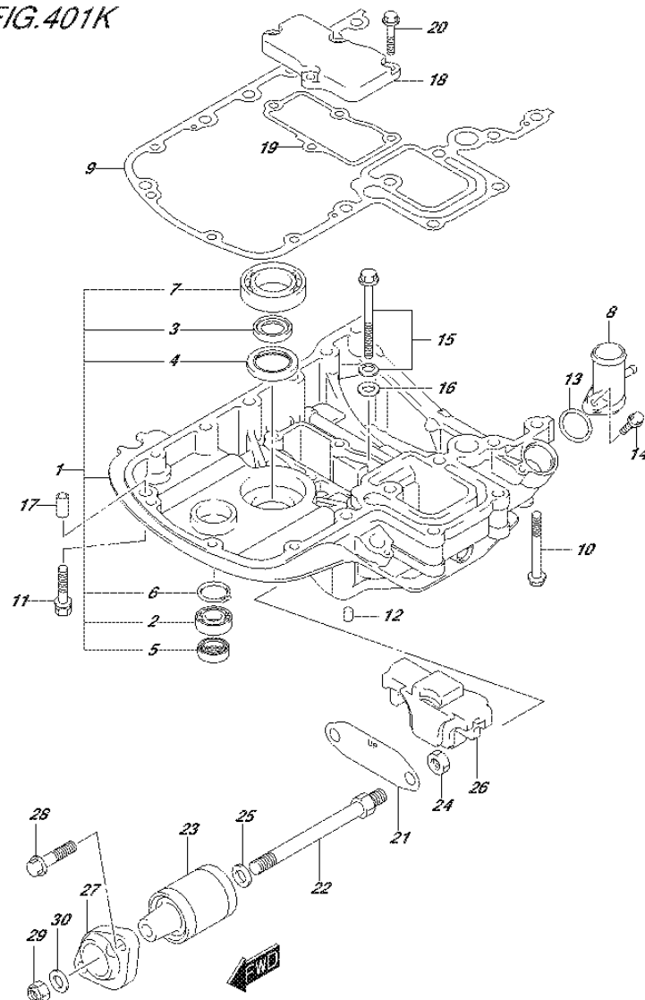
FIG.401K (2-G-8) ENGINE HOLDER (DF115AST E03)
