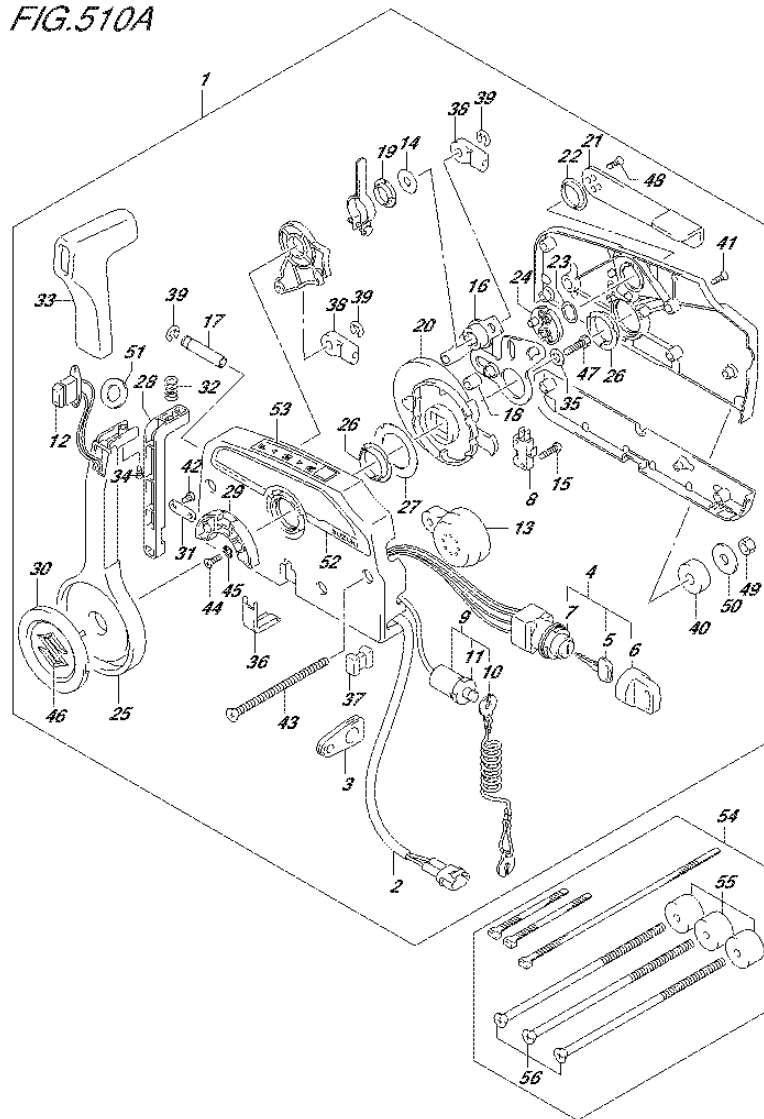
FIG.510A (3-E-6) OPT:REMOTE CONTROL (2) (DF100AT E11)
