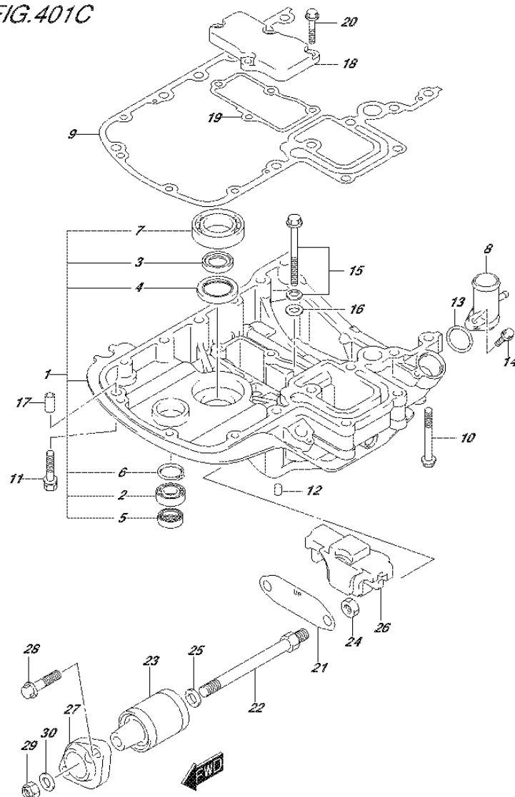
FIG.401C (2-F-15) ENGINE HOLDER (DF115AT E40)
