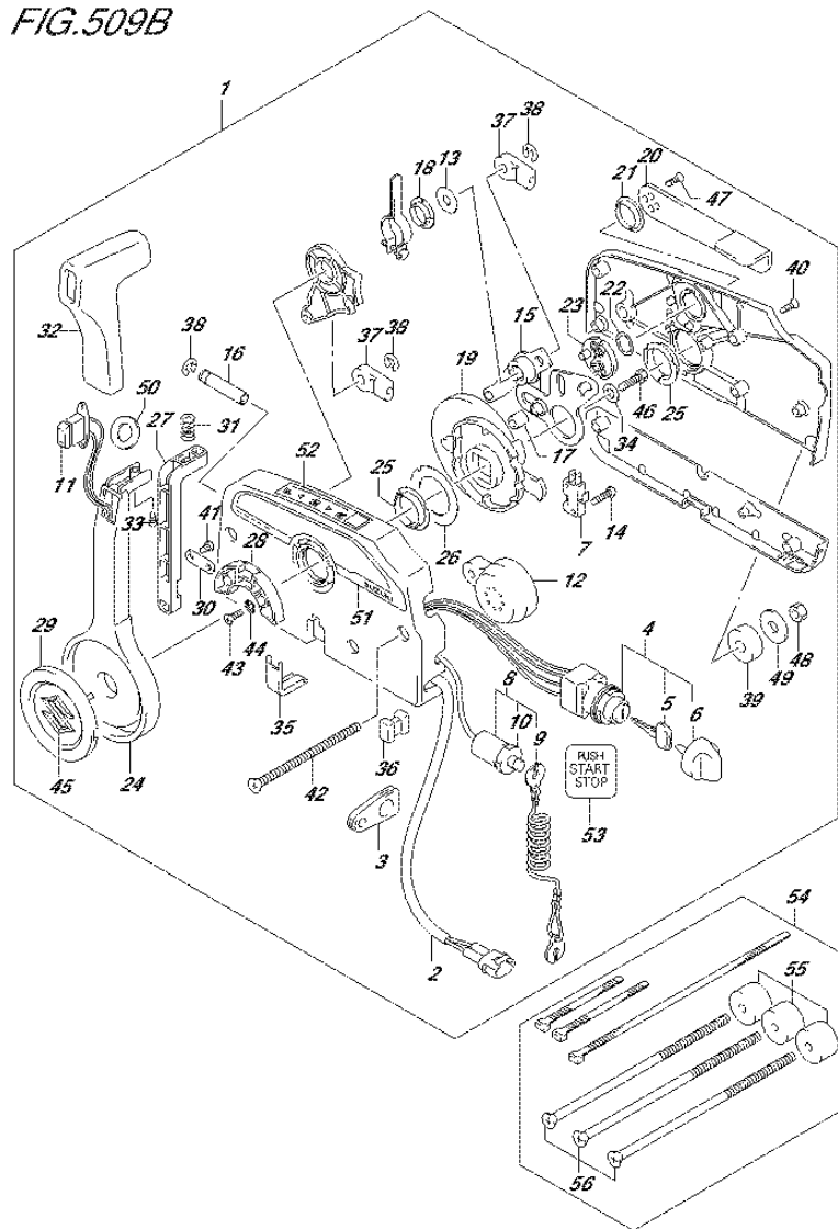
FIG.509B (3-D-8) OPT:REMOTE CONTROL (1) (DF115AT E11)
