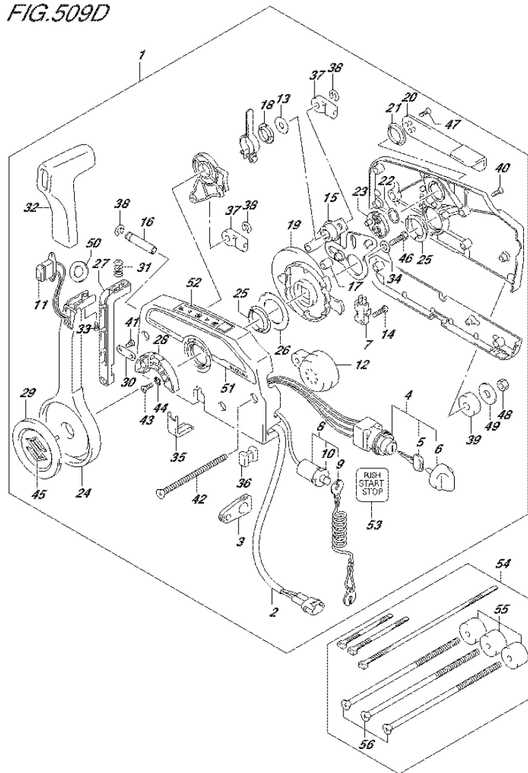
FIG.509D (3-D-14) OPT:REMOTE CONTROL (1) (DF140AT E11)
