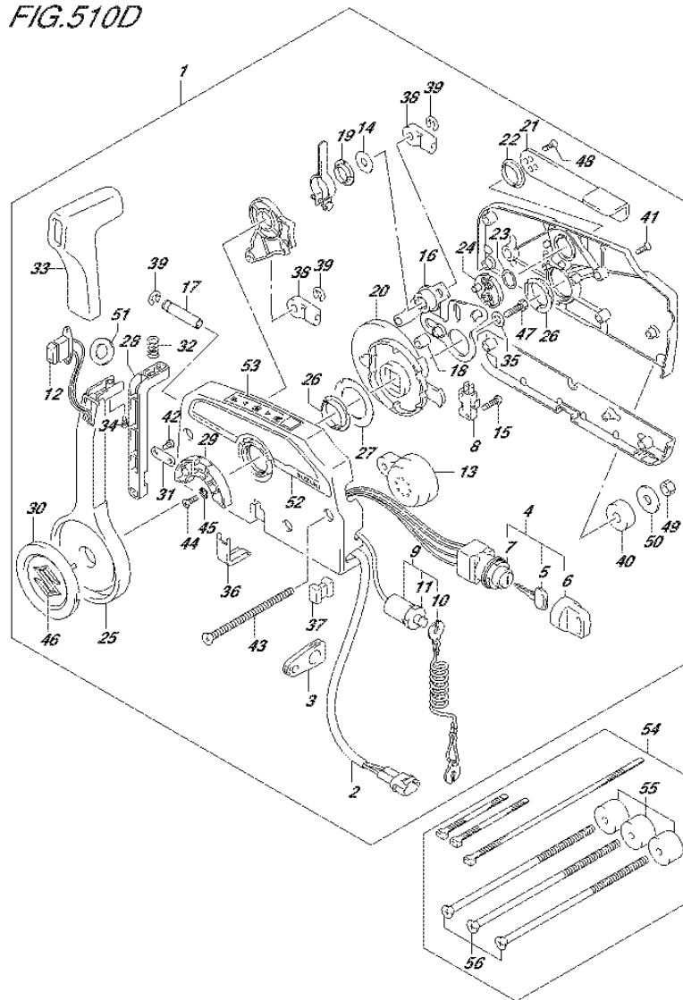
FIG.510D (3-E-15) OPT:REMOTE CONTROL (2) (DF115AZ E11)
