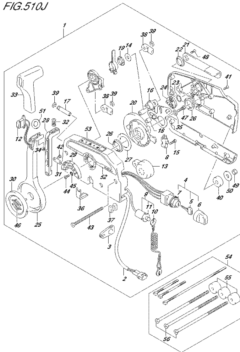
FIG.510J (3-G-2) OPT:REMOTE CONTROL (2) (DF140AZ E40)
