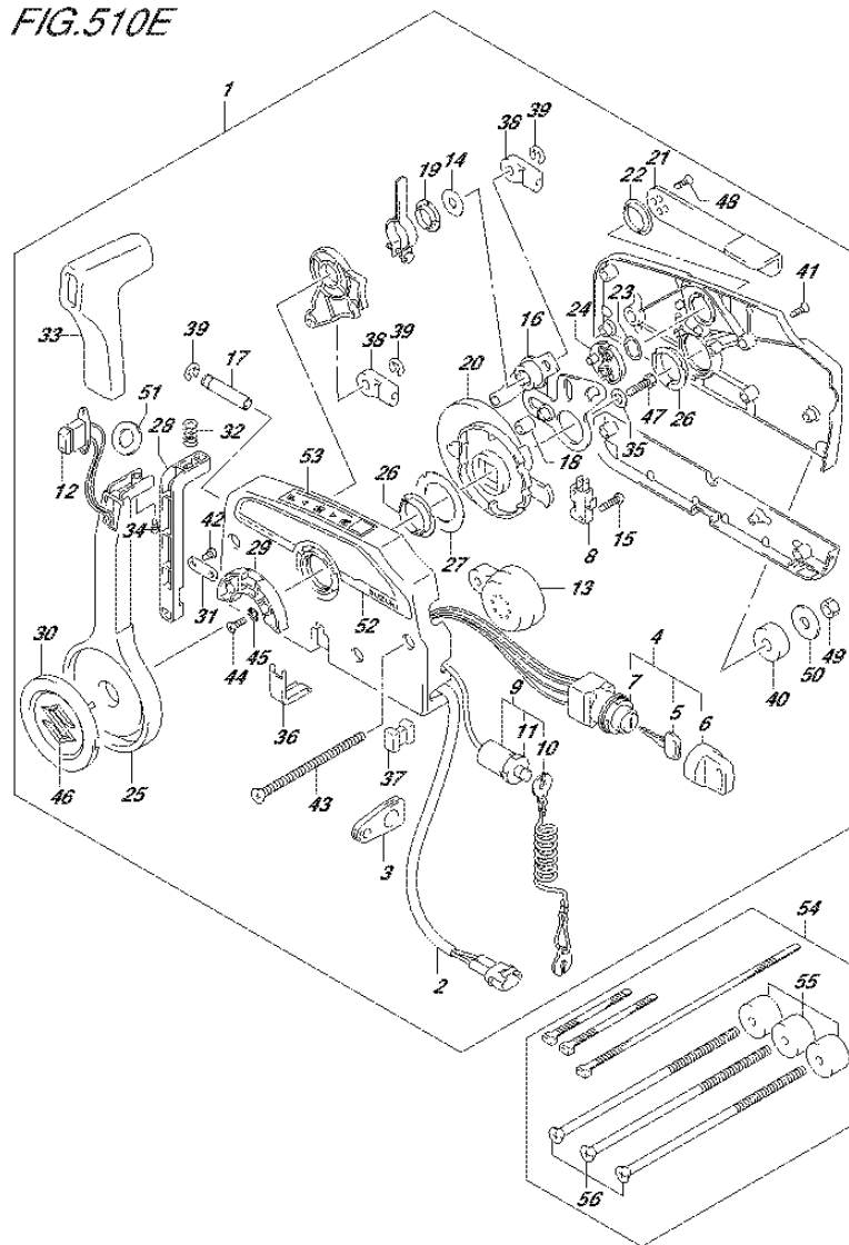
FIG.510E (3-F-4) OPT:REMOTE CONTROL (2) (DF115AZ E40)
