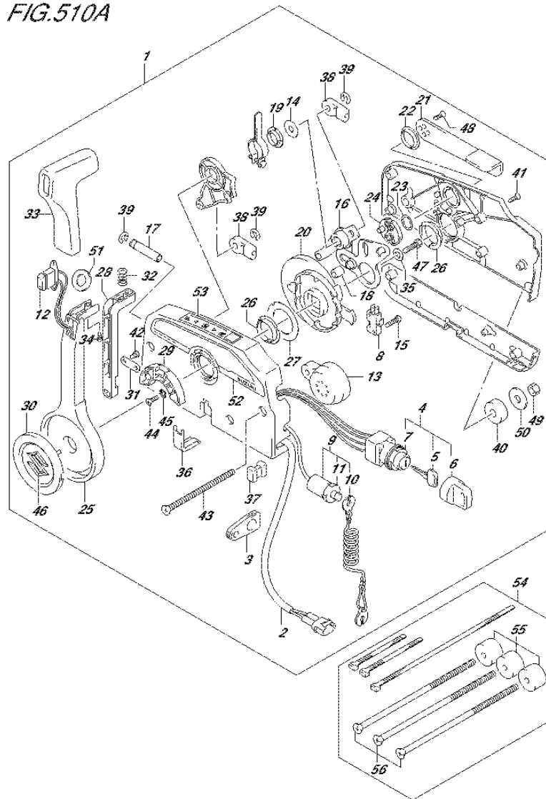
FIG.510A (3-E-7) OPT:REMOTE CONTROL (2) (DF100AT E11)
