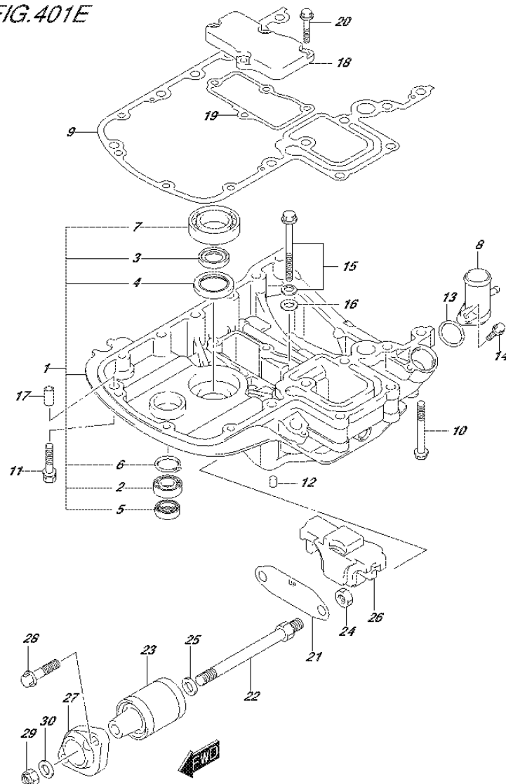
FIG.401E (2-G-3) ENGINE HOLDER (DF115AZ E40)
