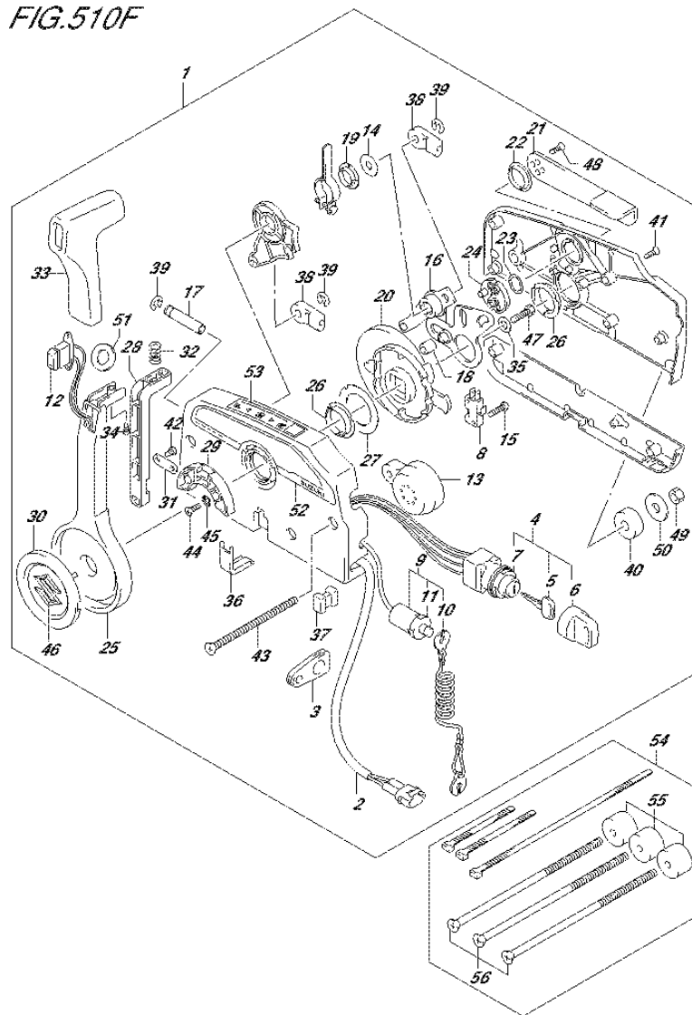
FIG.510F (3-F-7) OPT:REMOTE CONTROL (2) (DF140AT E11)
