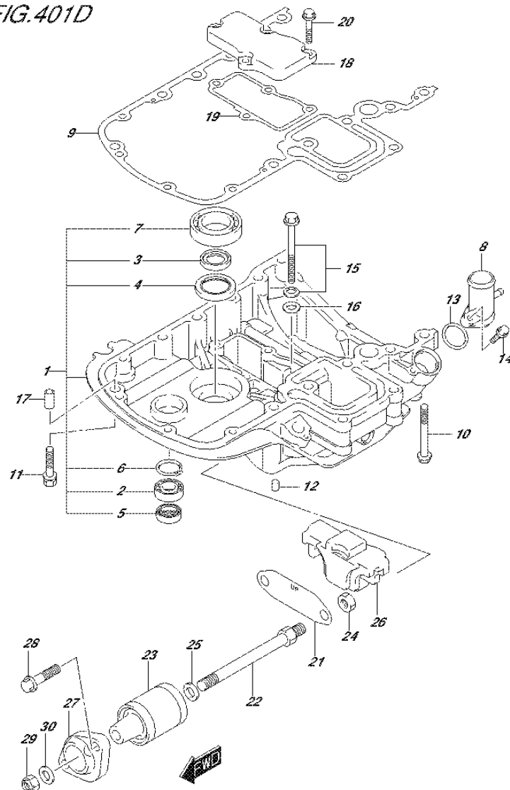
FIG.401D (2-G-2) ENGINE HOLDER (DF115AZ E11)
