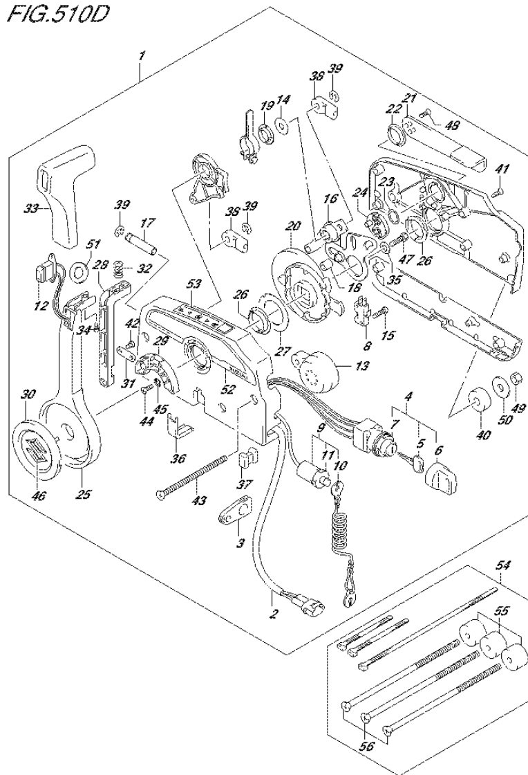
FIG.510D (3-E-14) OPT:REMOTE CONTROL (2) (DF115AZ E11)
