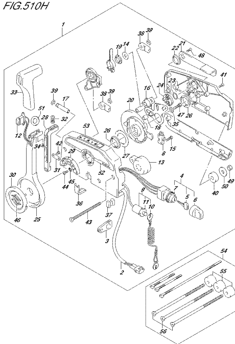
FIG.510H (3-F-12) OPT:REMOTE CONTROL (2) (DF140AZ E11)
