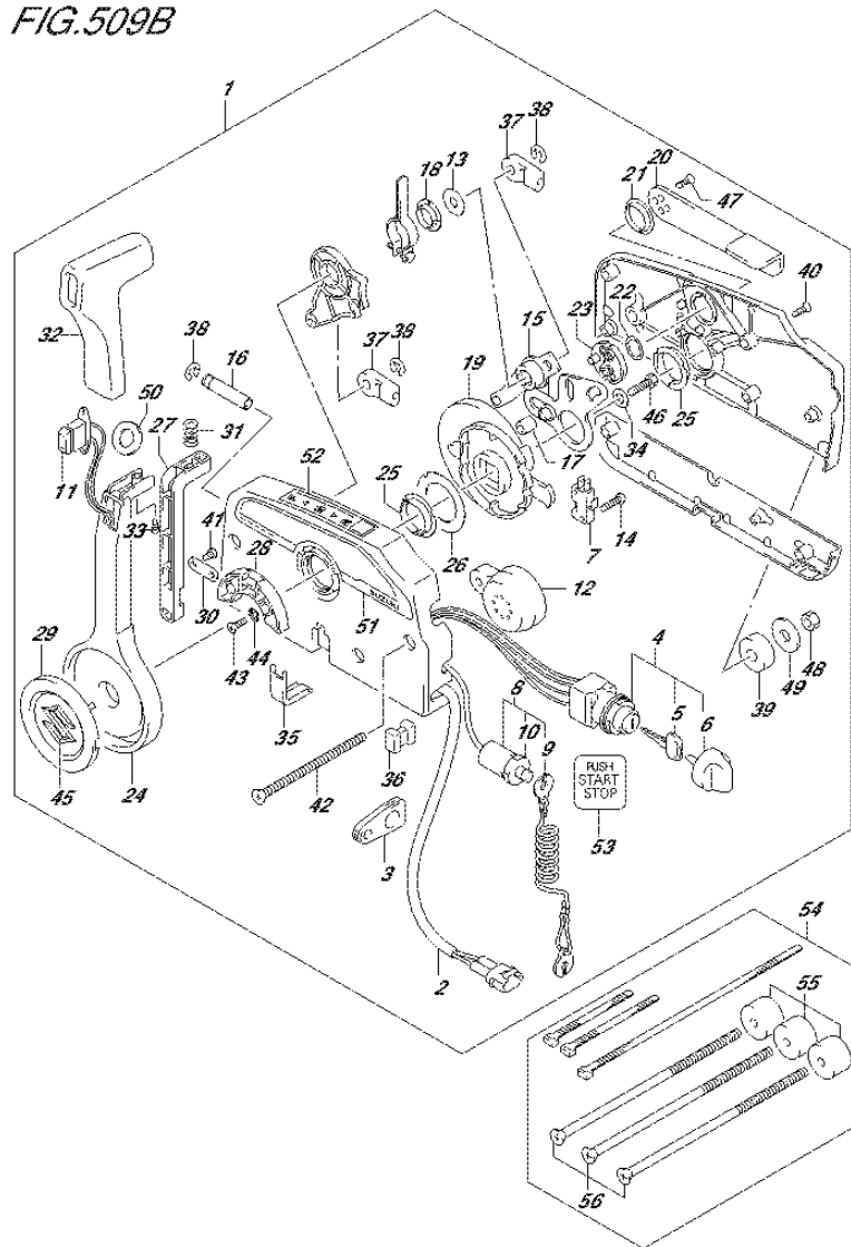
FIG.509B (3-D-7) OPT:REMOTE CONTROL (1) (DF115AT E11)
