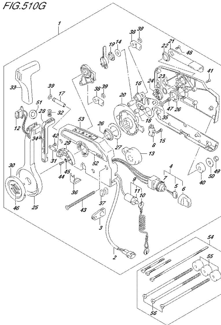
FIG.510G (3-F-10) OPT:REMOTE CONTROL (2) (DF140AT E40)
