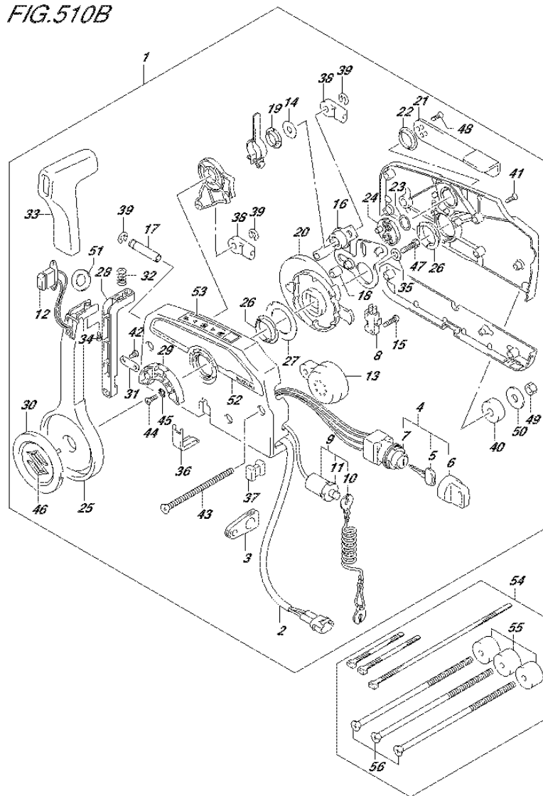
FIG.510B (3-E-9) OPT:REMOTE CONTROL (2) (DF115AT E11)
