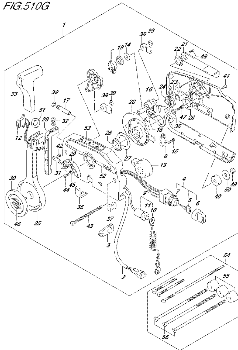
FIG.510G (3-F-9) OPT:REMOTE CONTROL (2) (DF140AT E40)
