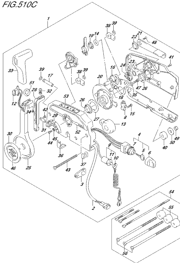
FIG.510C (3-E-11) OPT:REMOTE CONTROL (2) (DF115AT E40)
