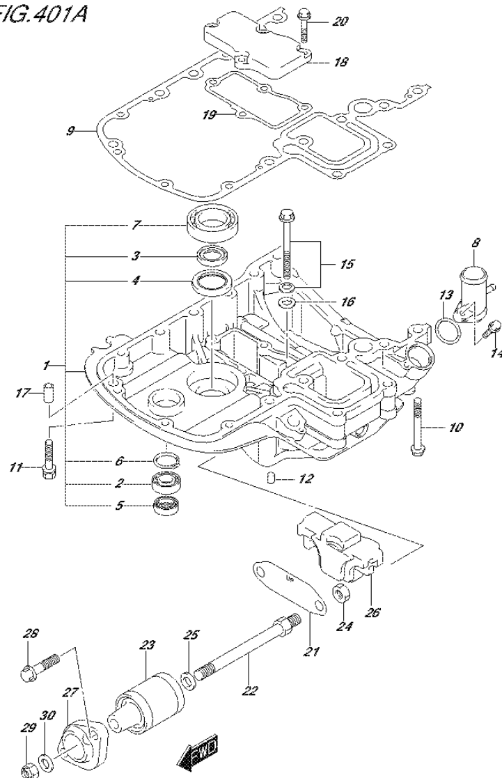
FIG.401A (2-F-13) ENGINE HOLDER (DF100AT E11)
