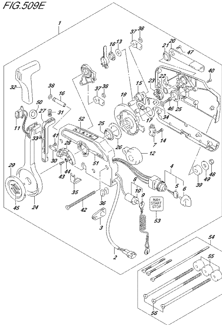
FIG.509E (3-E-3) OPT:REMOTE CONTROL (1) (DF140AZ E11)
