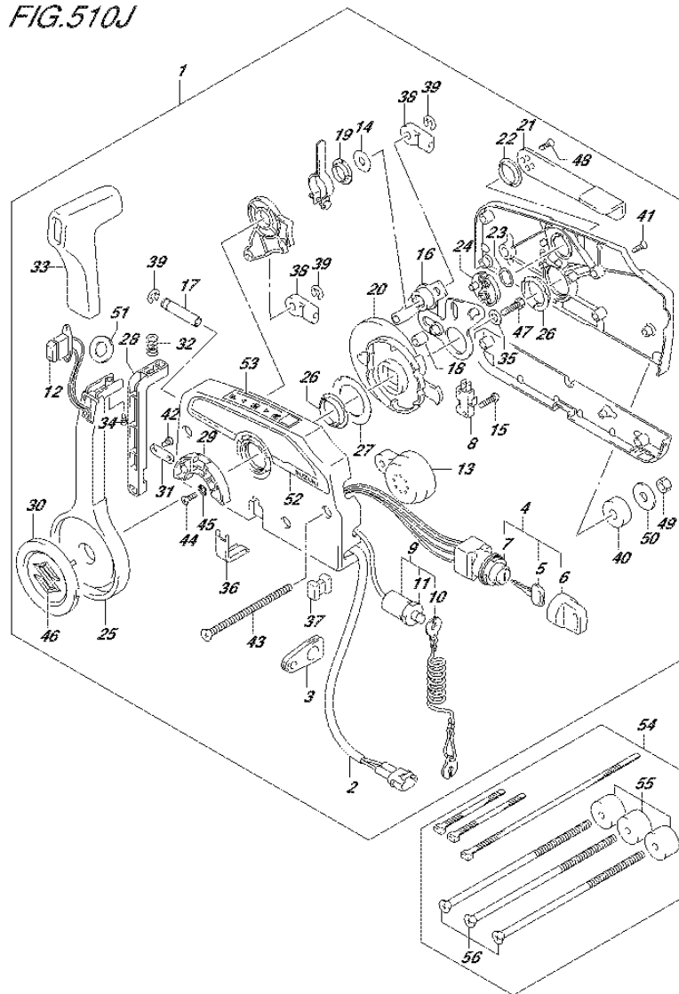
FIG.510J (3-G-3) OPT:REMOTE CONTROL (2) (DF140AZ E40)
