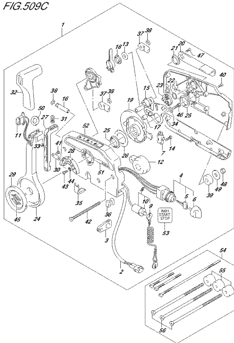
FIG.509C (3-D-10) OPT:REMOTE CONTROL (1) (DF115AZ E11)
