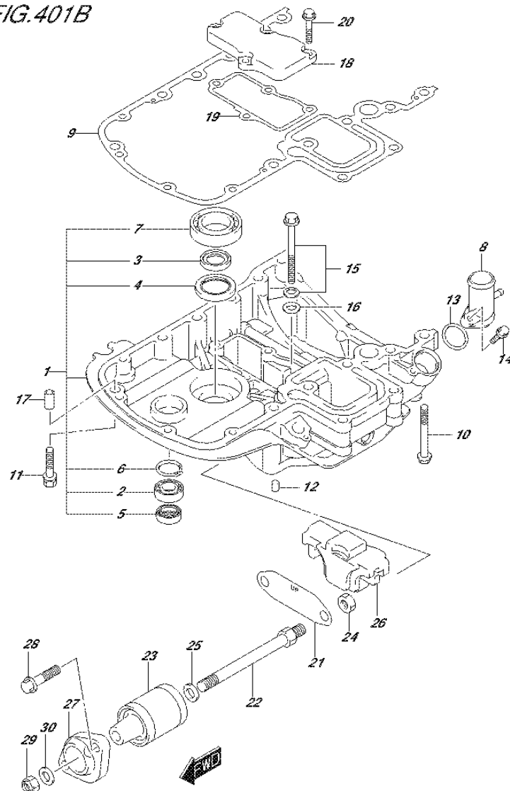
FIG.401B (2-F-14) ENGINE HOLDER (DF115AT E11)
