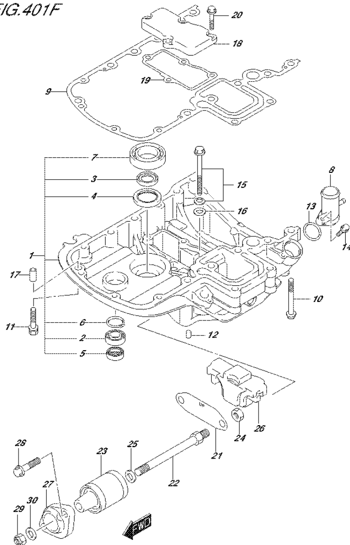
FIG.401F (2-G-4) ENGINE HOLDER (DF140AT E11)
