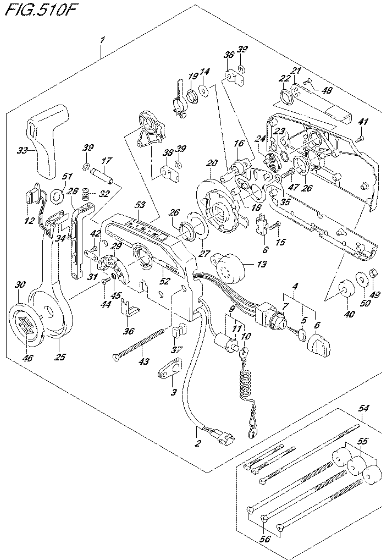
FIG.510F (3-F-8) OPT:REMOTE CONTROL (2) (DF140AT E11)
