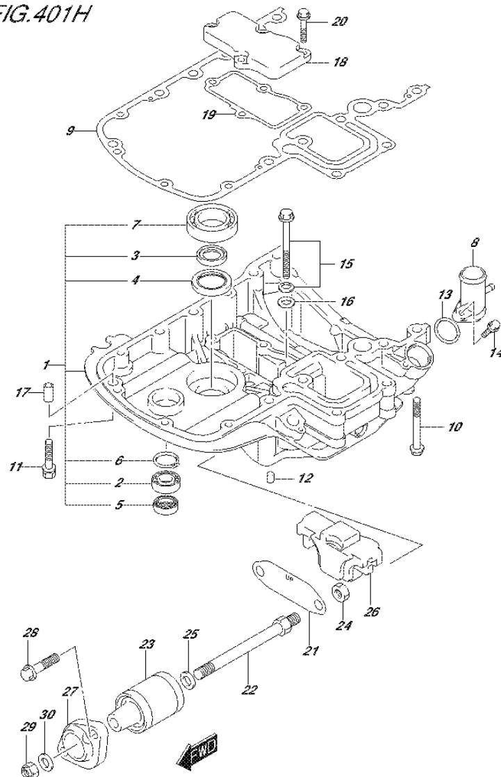
FIG.401H (2-G-6) ENGINE HOLDER (DF140AZ E11)
