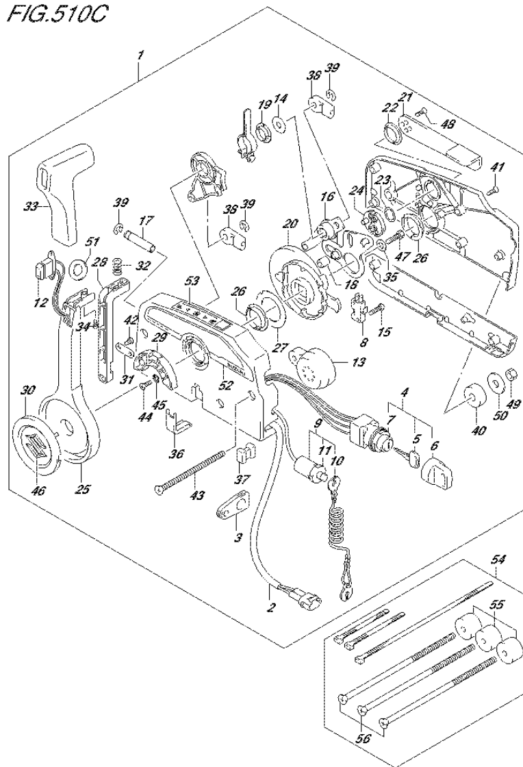
FIG.510C (3-E-12) OPT:REMOTE CONTROL (2) (DF115AT E40)
