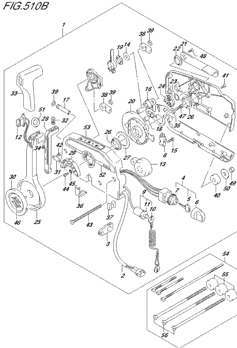
FIG.510B (3-E-10) OPT:REMOTE CONTROL (2) (DF115AT E11)
