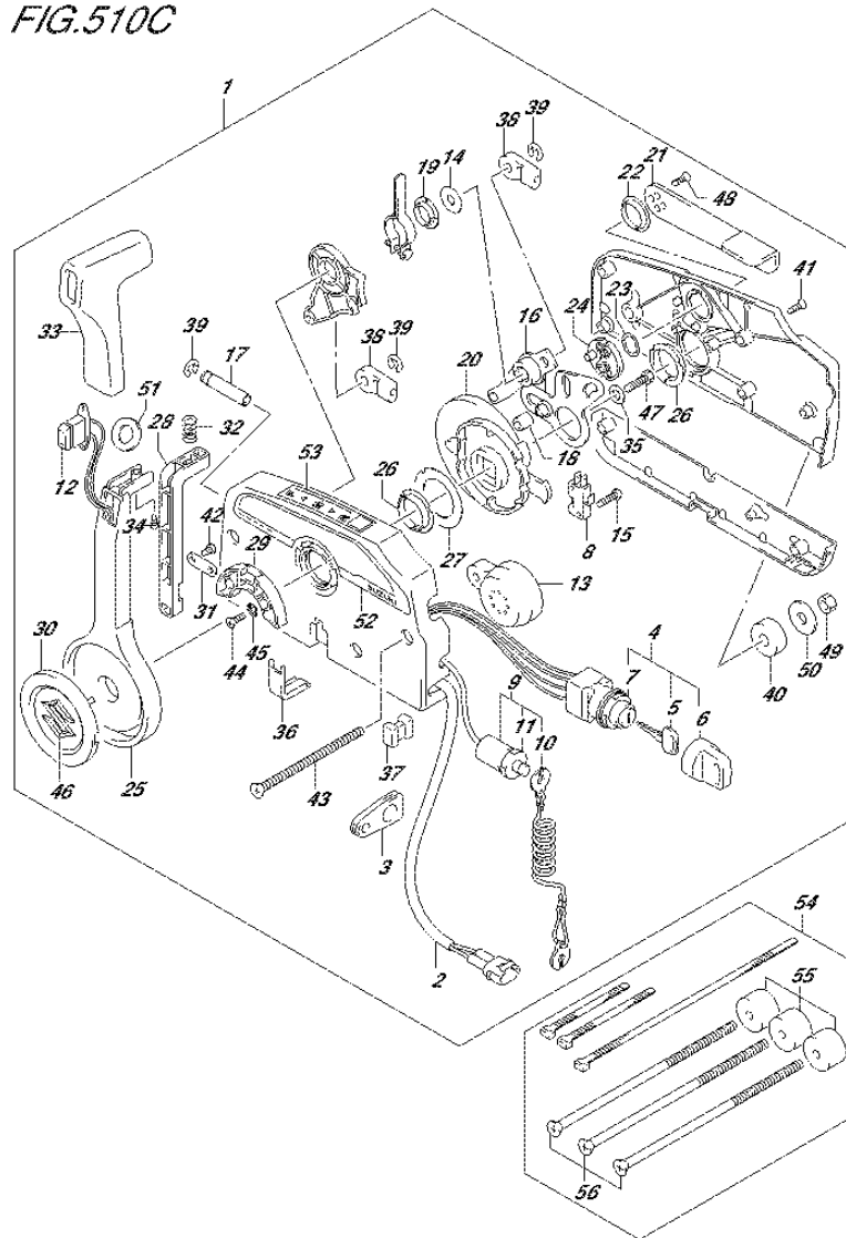
FIG.510C (3-E-13) OPT:REMOTE CONTROL (2) (DF115AT E40)
